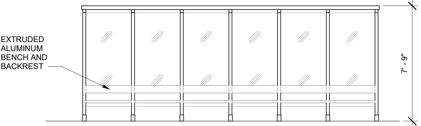
2 002 1/4" = 1'-0" PREFABRICATED SMOKERS CANOPY ELEVATION - FRONT
