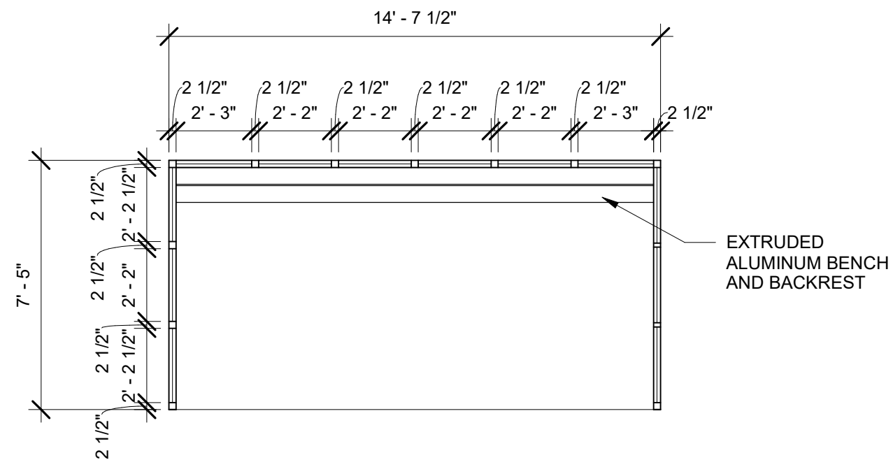
PREFABRICATED DROP-OFF CANOPY PLAN
