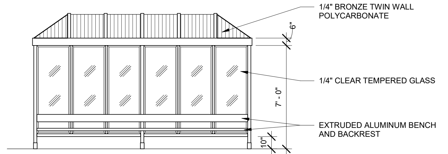
PREFABRICATED DROP-OFF CANOPY ELEVATION - FRONT
